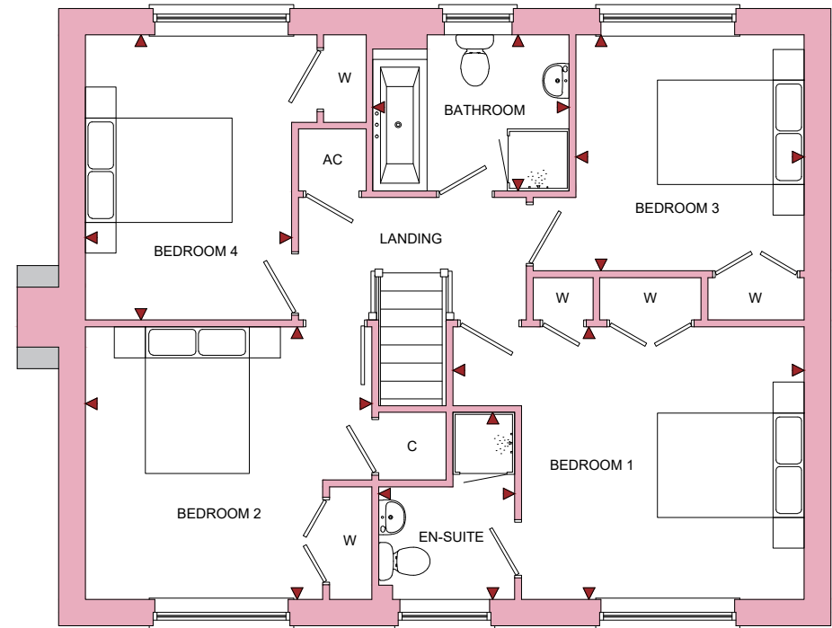
FIRST FLOOR
